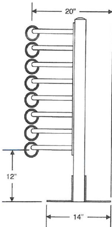
Spartan 7 7 skateboard capacity Floor Mount Single Sided Use
